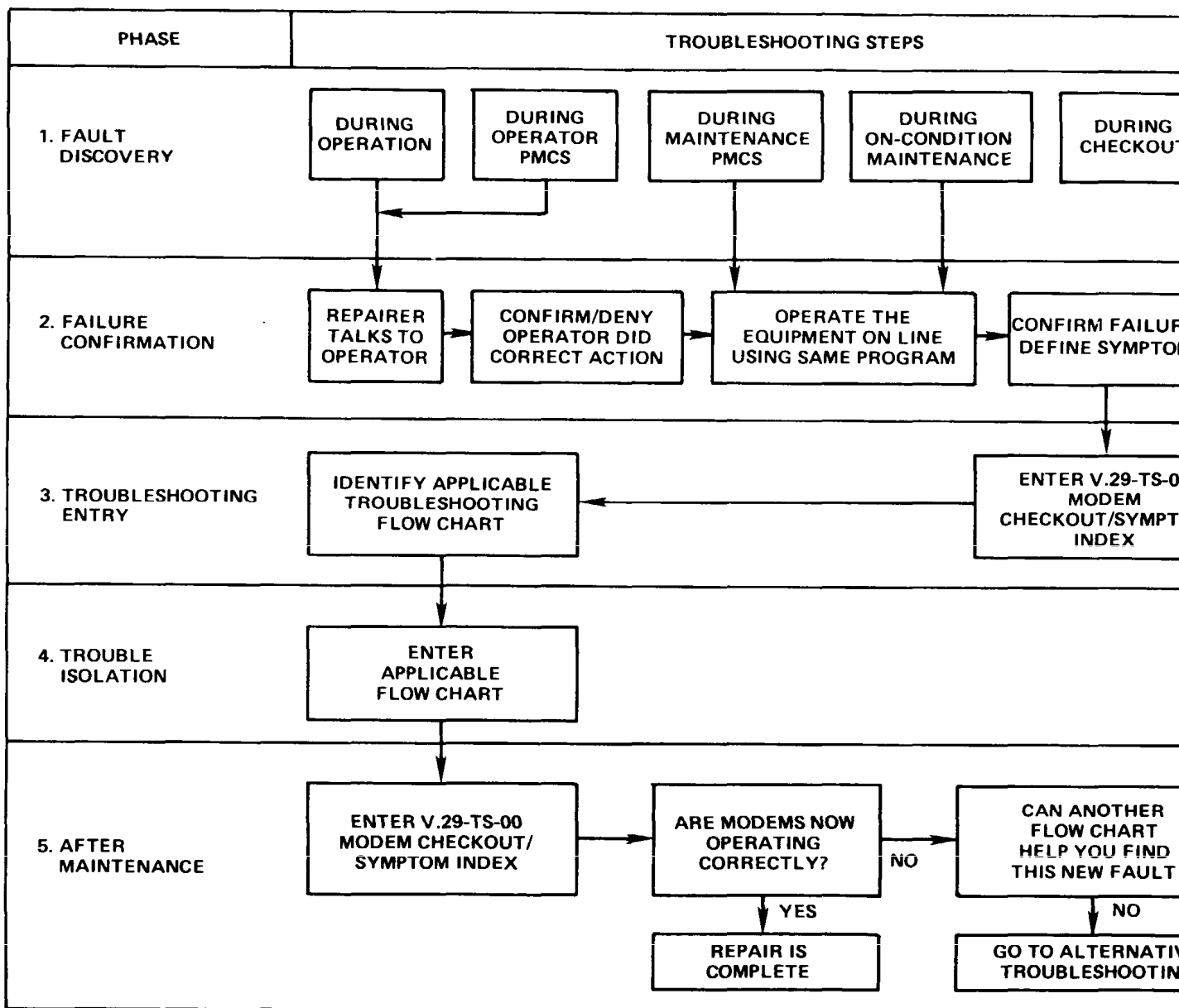
Figure 4-1. Troubleshooting Phases
