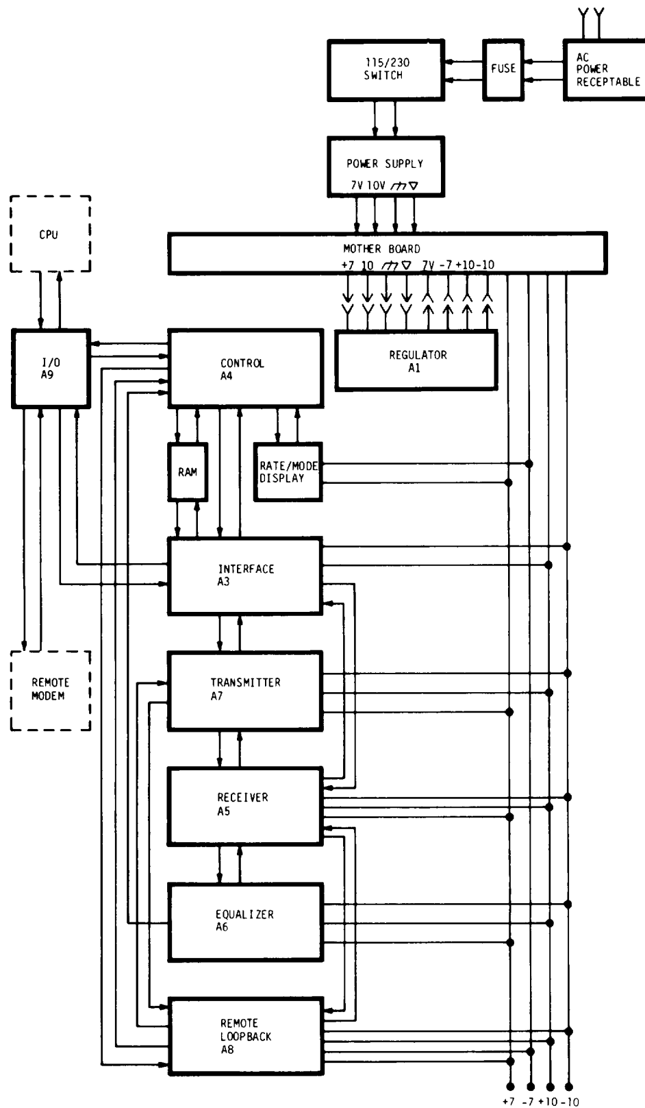
Figure 2-4. V.29 Modem Assembly Functional Block Diagram
